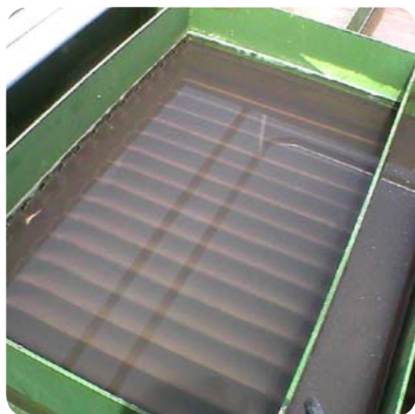
Top of clarifier showing water quality using existing treatment
