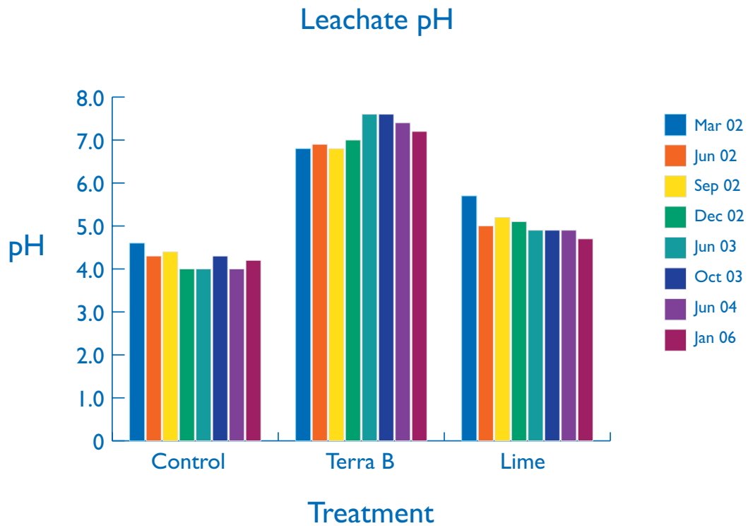
Figure 3. Acid neutralisation in a waste rock dump using TerraB™ reagent and lime.
