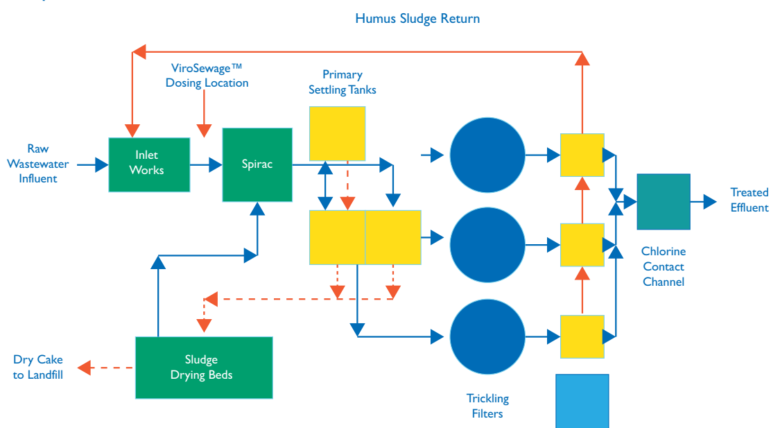
Layout of Sewage Treatment Plant (STP) at RAAF Base Amberley
