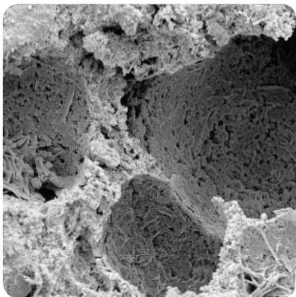
A Scanning Electron Microscopic (SEM) image of the interconnected pore space of the ViroFilter™ pellets
