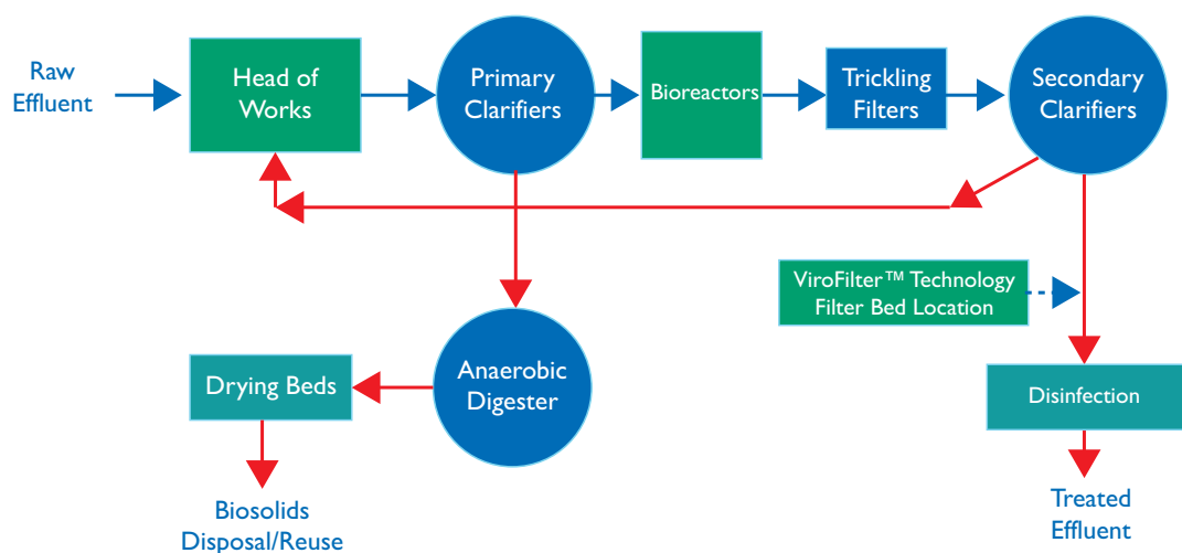
FIGURE 3: THE VIROFILTER™ BED LOCATION AT KIRK SMEATON
